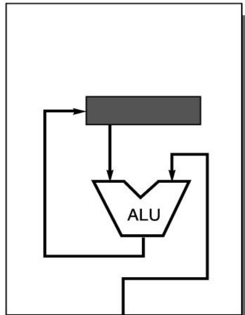
(b) Accumulator
