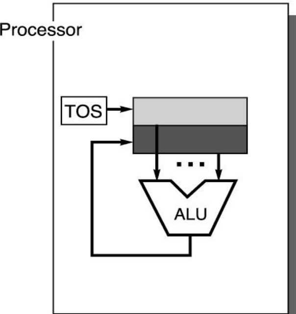
(a) Stack
